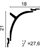
C991 + 2x P9900
